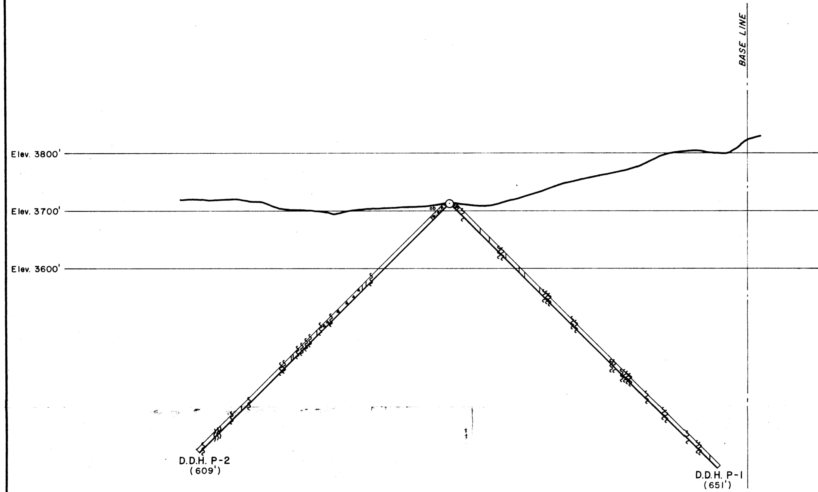
SECTION A-A' (LOOKING NORTH)
