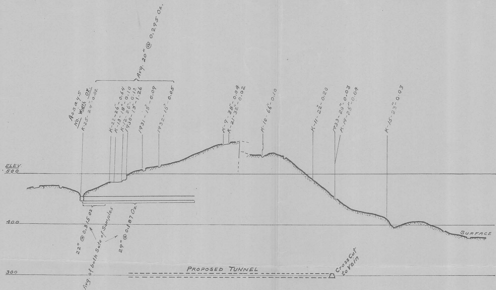
LONGITUDINAL SECTION ON C VEIN.
