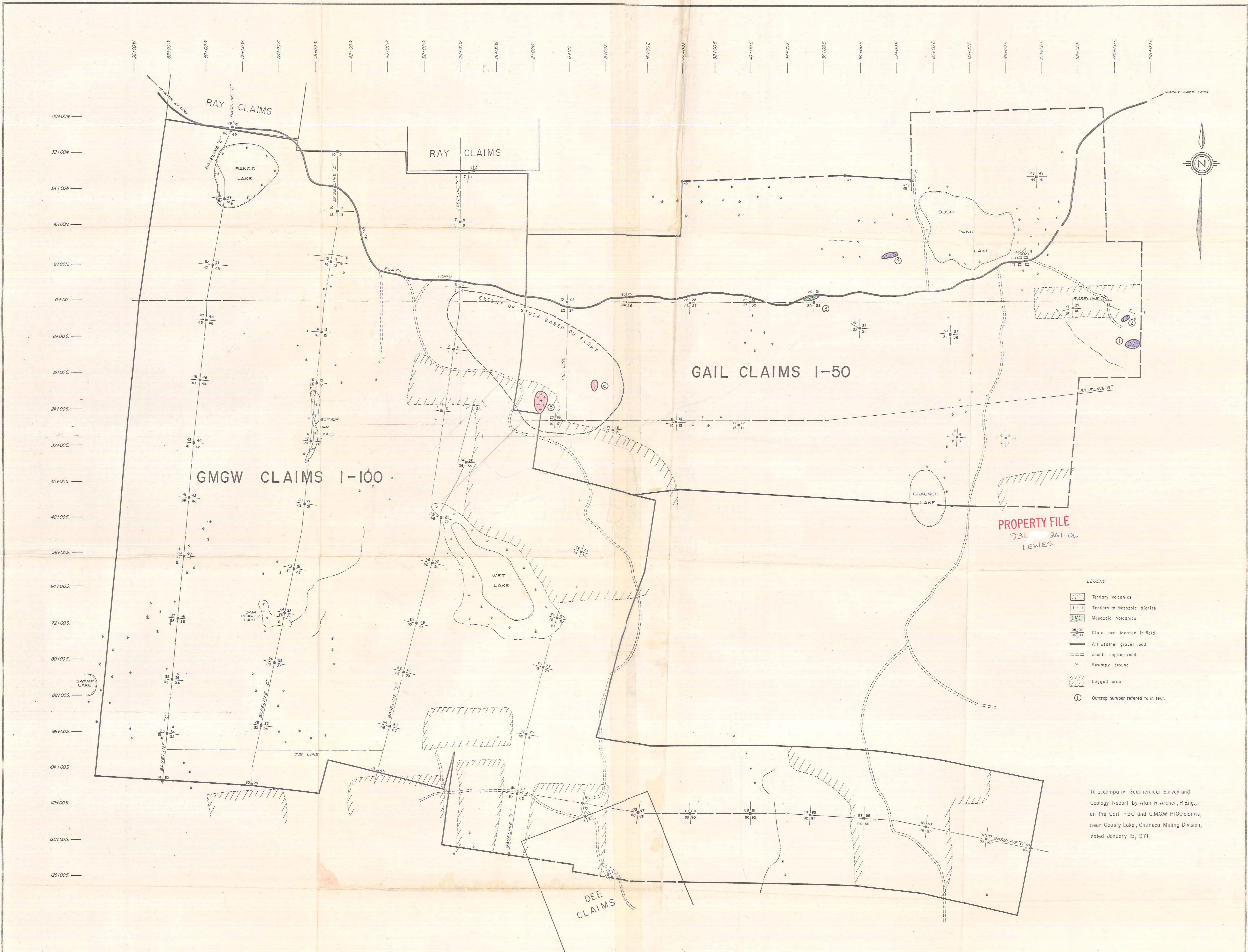
FIG. 2 ARCHER CATHRO & ASSOCIATES LTD. GEOLOGY AND CLAIM POST LOCATIONS LEWES RIVER MINES LTD. GOOSLY LAKE PROPERTY, HOUSTON, B.C.
