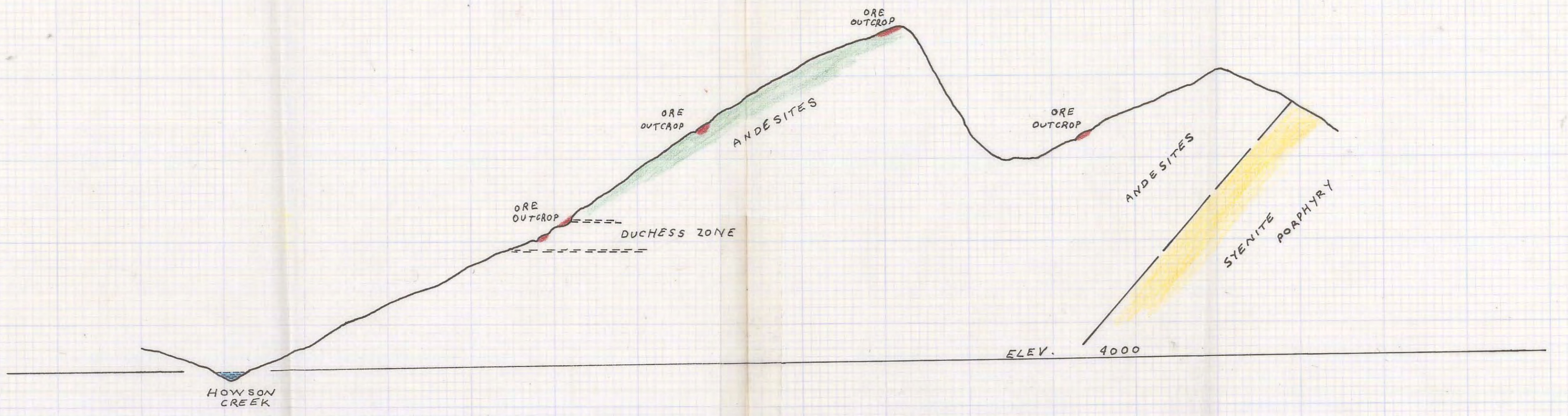
LONGITUDINAL SECTION (LOOKING WEST) 1" = 500'
