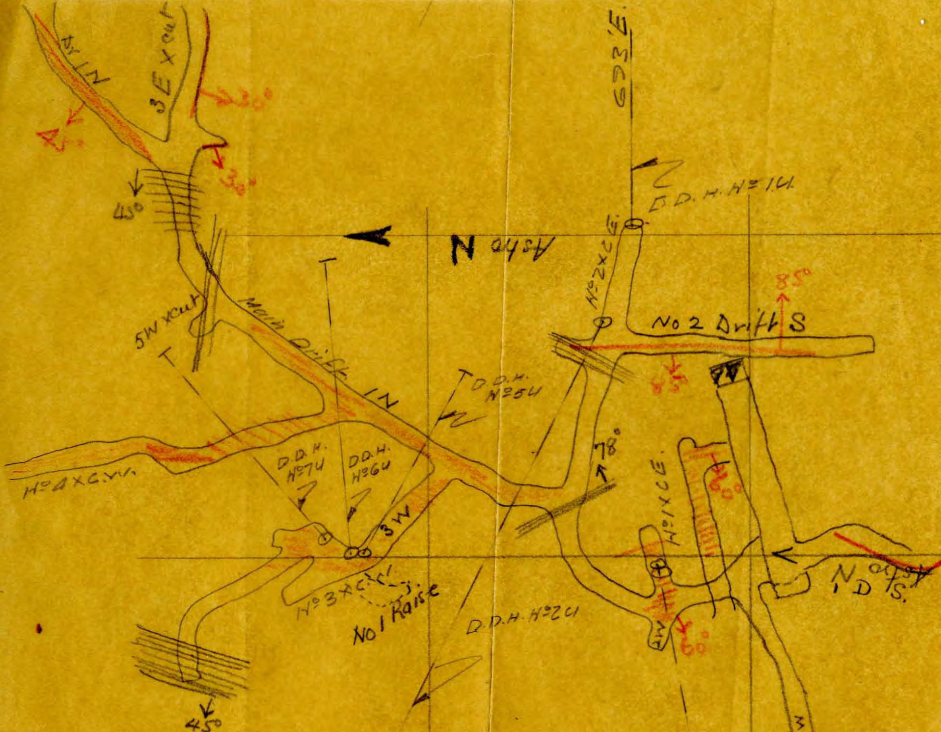
SKETCH of Under-ground diamond drill holes. Topley Richfield Mines Ltd Scale 1" = 30'
