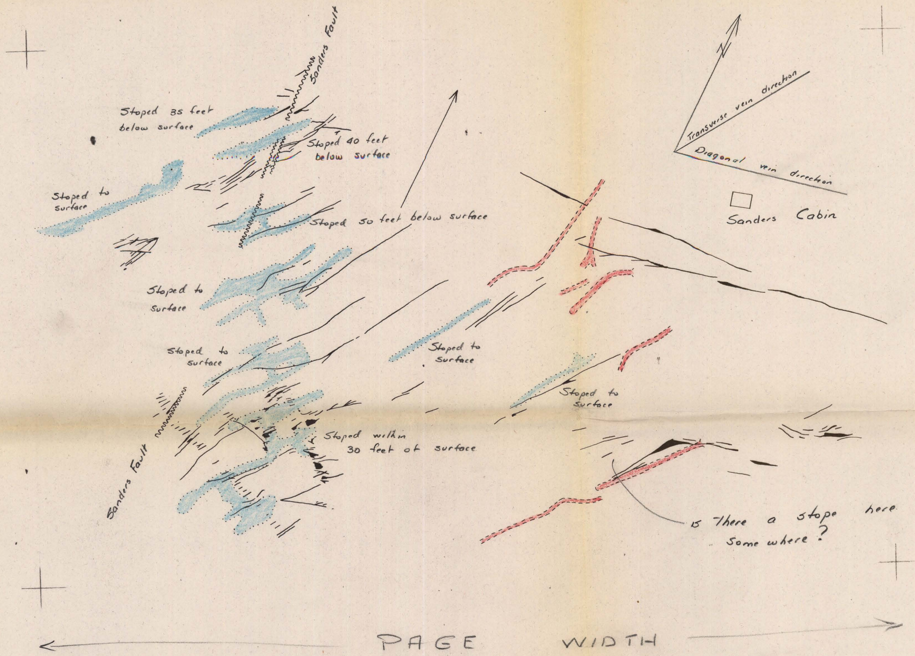
Figure 4. Reduction \pm 3:1 Surface workings on the Sanders zone shown in relation to the veins developed on the 900 level of the Cariboo Gold Quartz mine, and to the stopes between 900 level and the surface.
