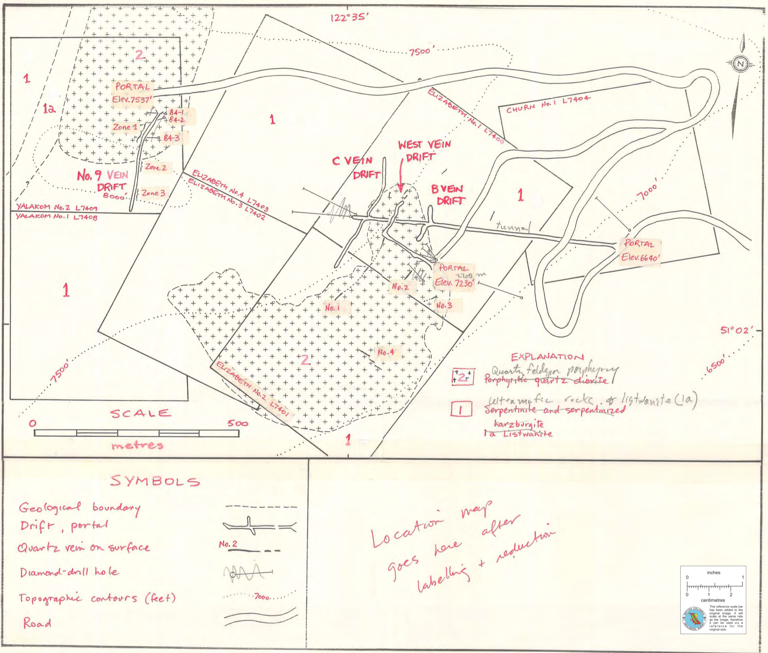
Figure 2/00-1 Location and geology of the Elizabeth-Yalakom prospect (includes information from: Bralorne Mines Ltd. (1953), Leech (1948), McCammon (19466), and Thompson (1957a,b)).
