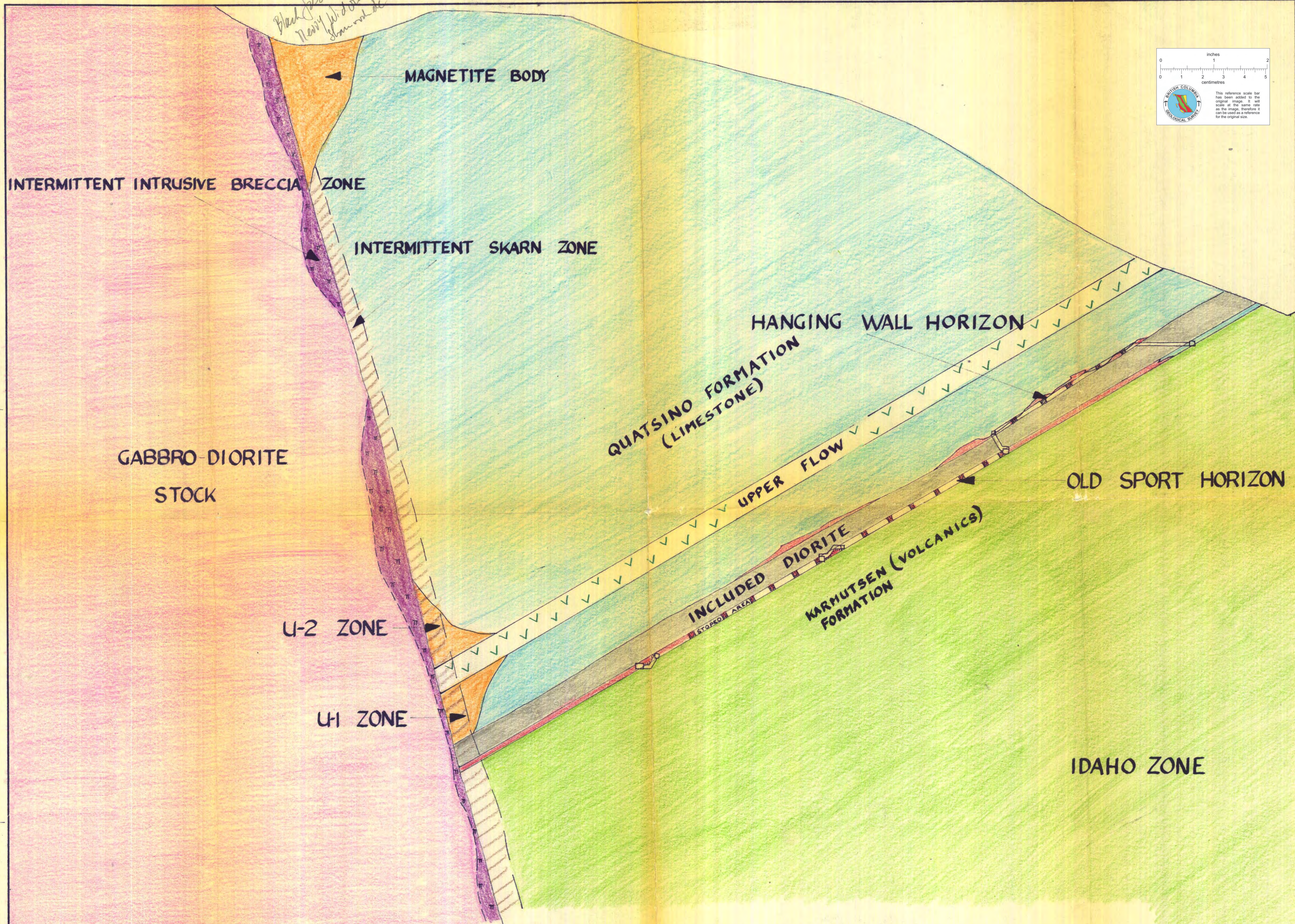
COAST COPPER - BENSON LAKE MINES, GENERALISED GEOLOGICAL SECTION
