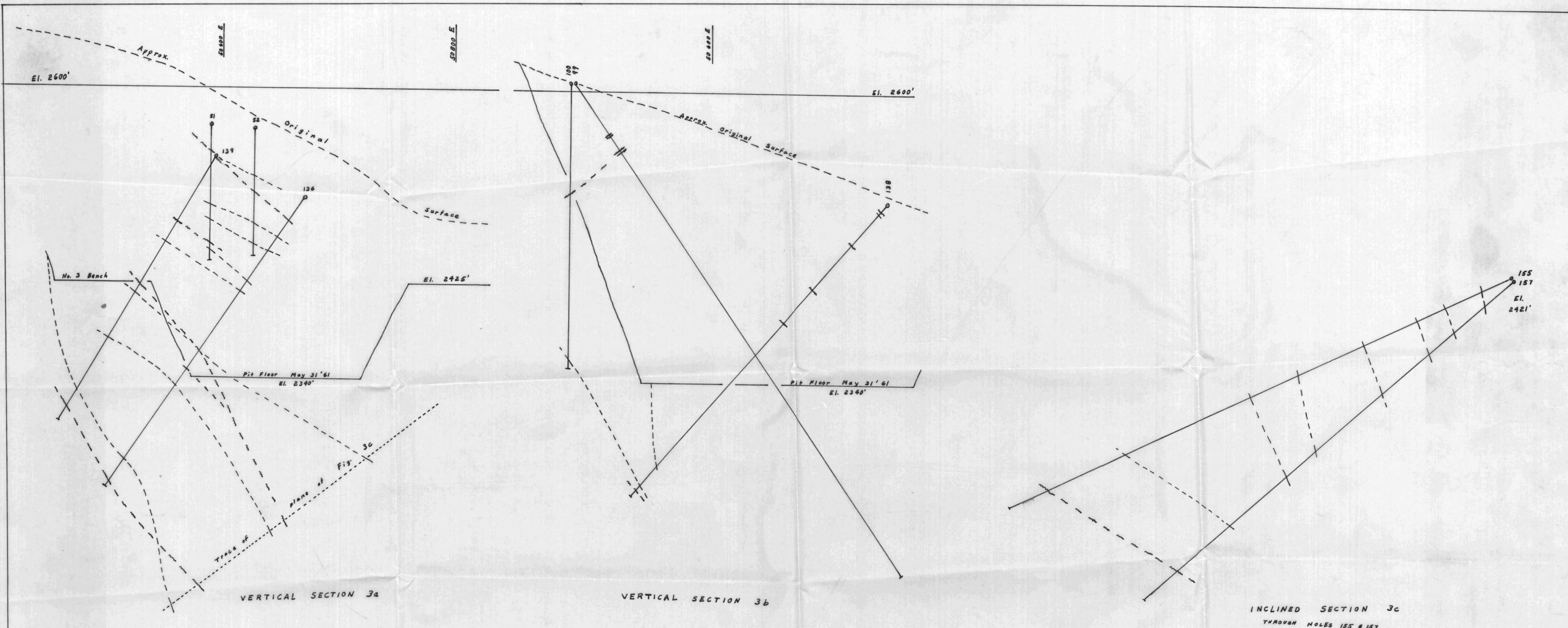
Figure 3 SECTIONS THROUGH DRILL HOLES SHOWN ON FIG. 2 Scale: Feet Legend on Fig. 1
