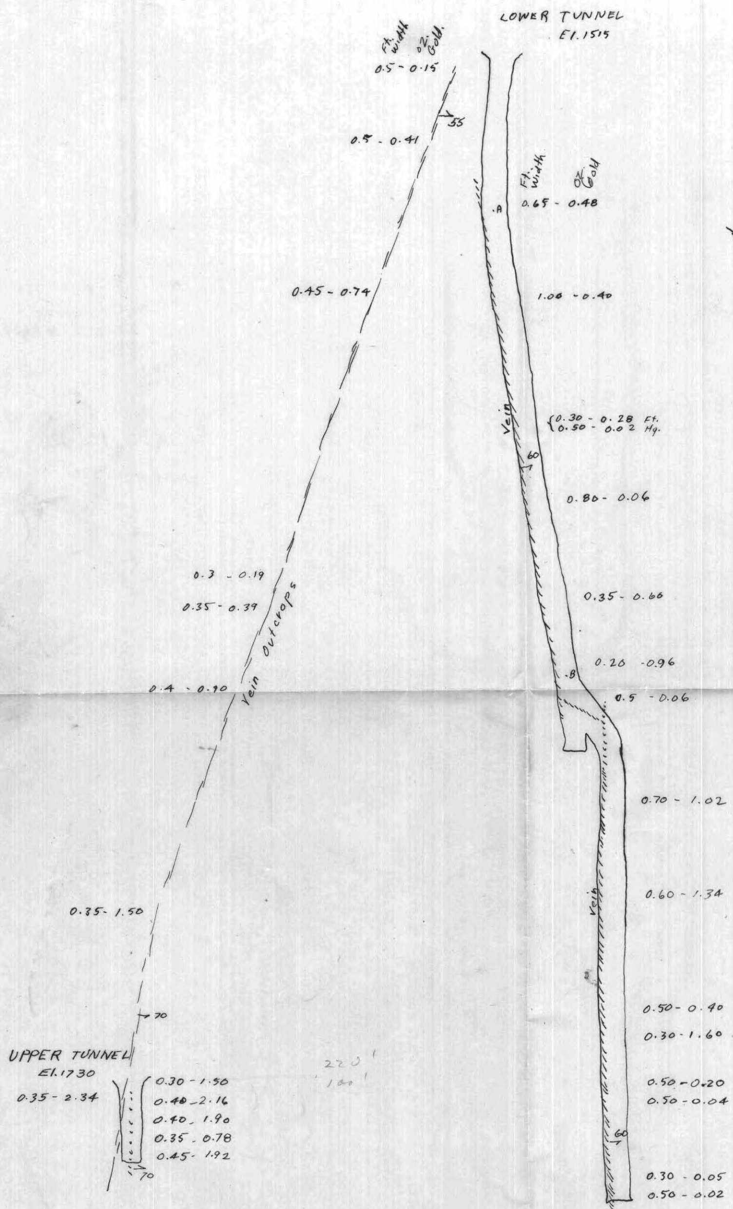
PLAN OF WORKINGS SCALE: 1" = 20'
