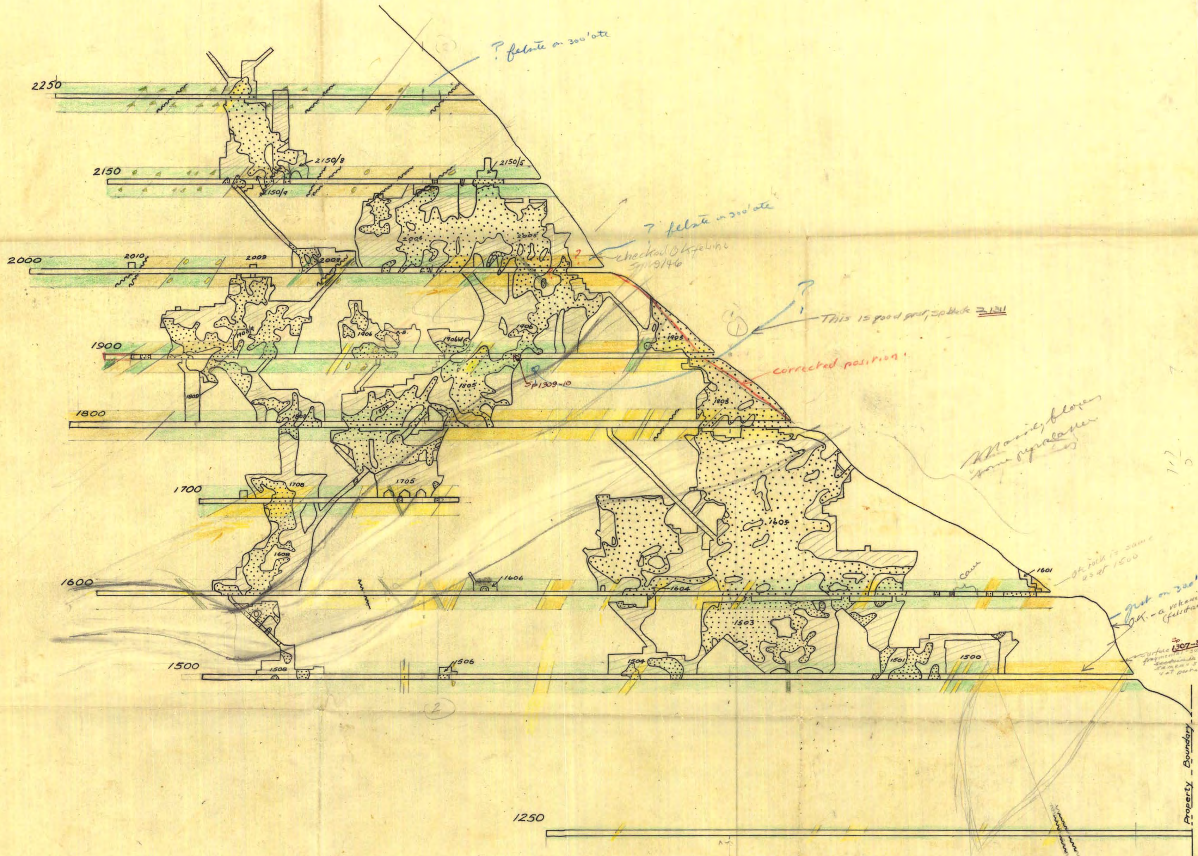
MOUNT ZEBALLOS GOLD MINES STOPE PROFILE SHOWING ORE SHOOTS
