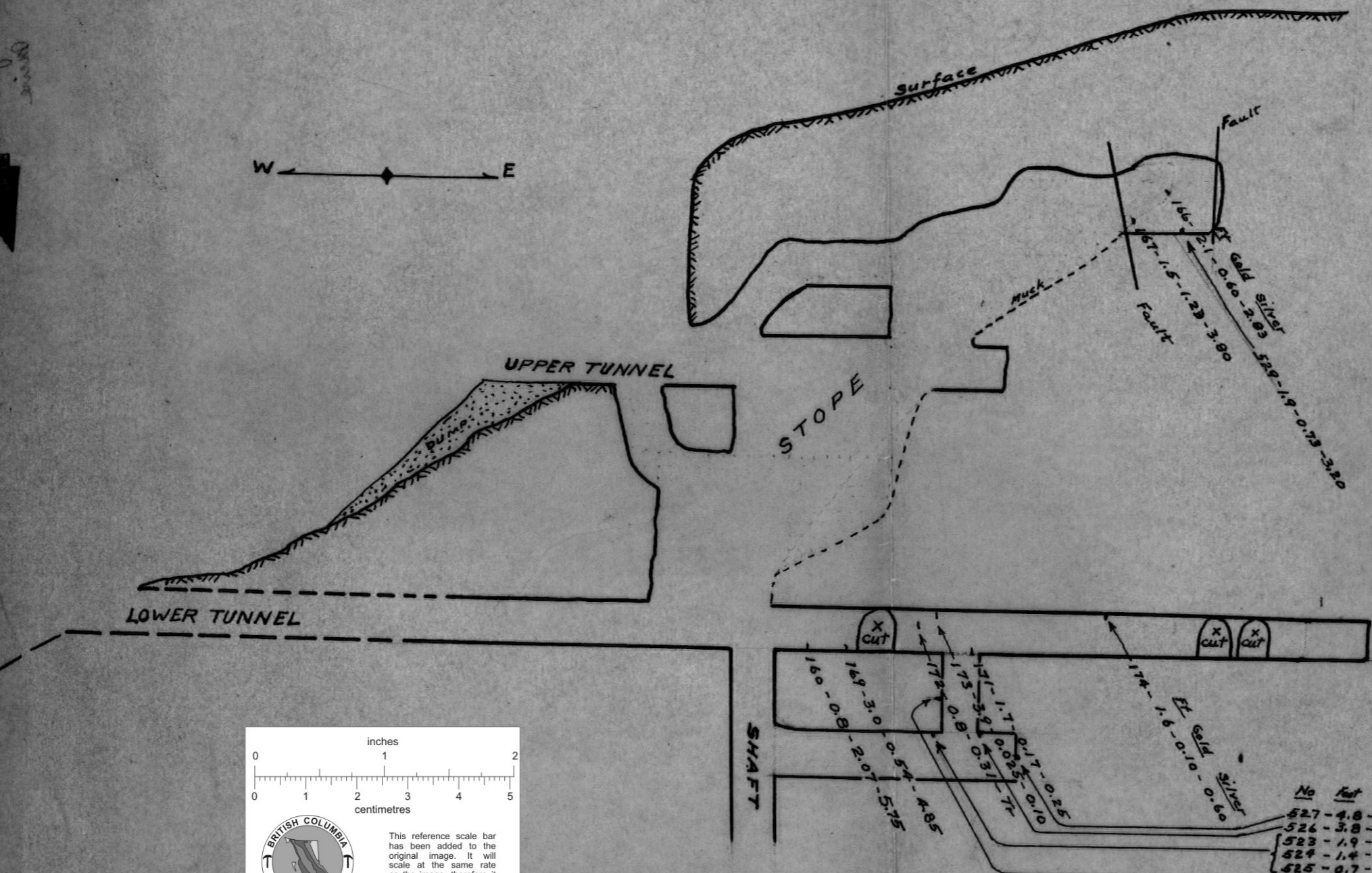
LOUGHBOROUGH GOLD MINES LTD SECTIONS THROUGH TUNNELS SCALE: 1"=20'
