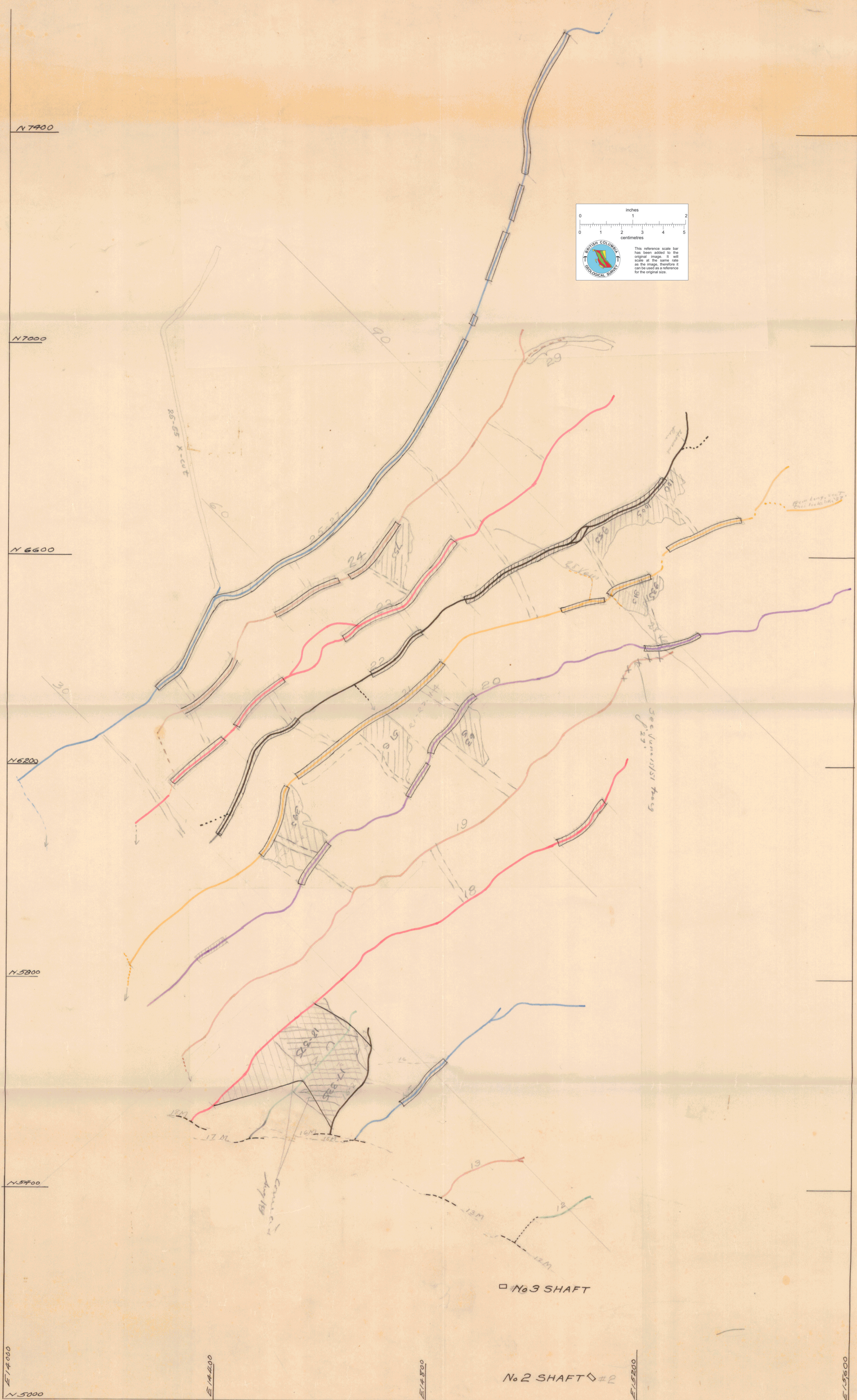
Fig. Pioneer. Plan of "27" vein, showing drifts, ore-blocks & stoped areas. This unit has been brought up to date with other drawings of 27. (June 1951)
