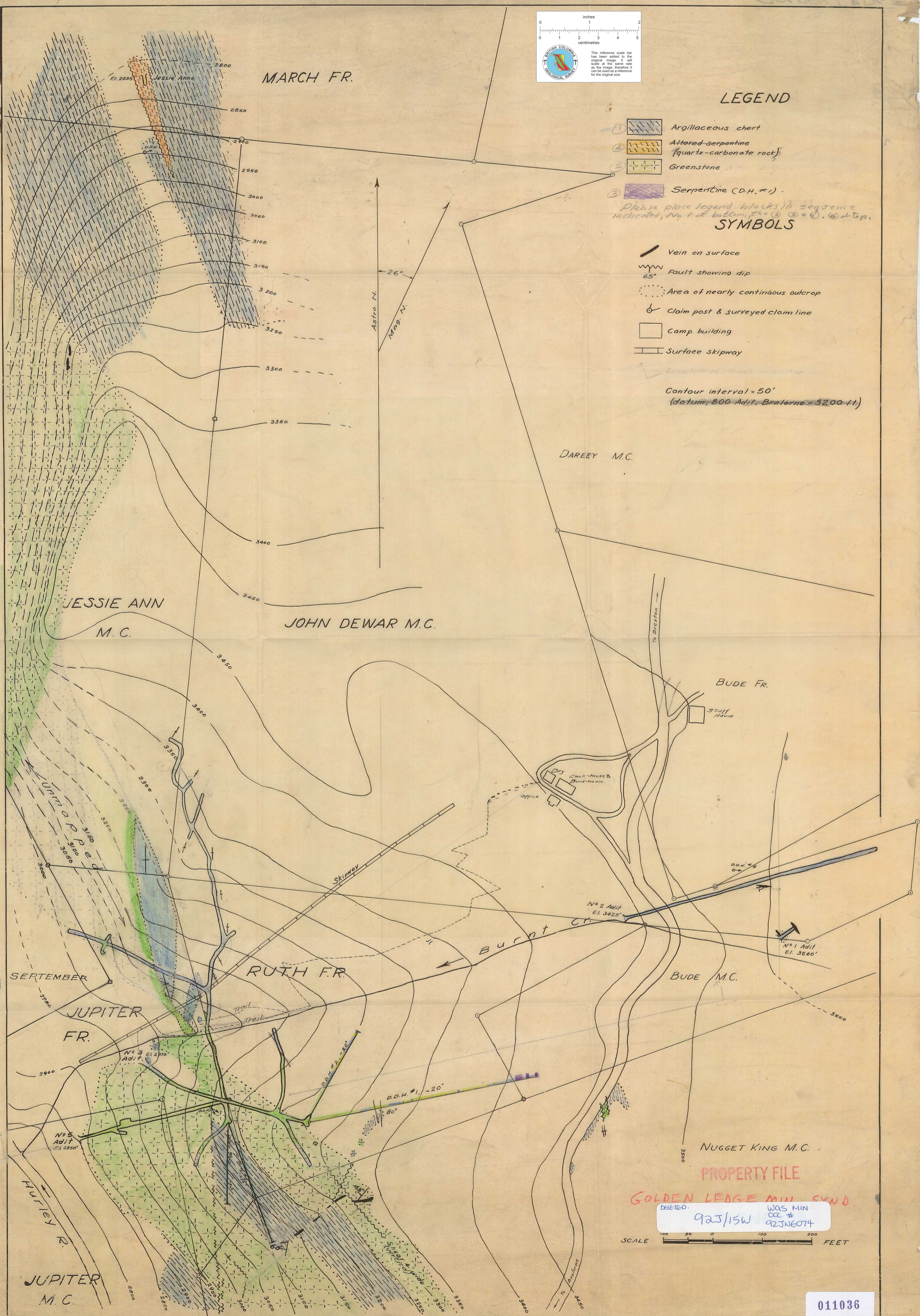
Fig. Surface geology, underground workings, diamond drill holes, Golden Ledge Mining Agreement, Daley Mine. Contour interval 50 feet. Datum = 800 Adit, Bralorne = 3200 feet.
