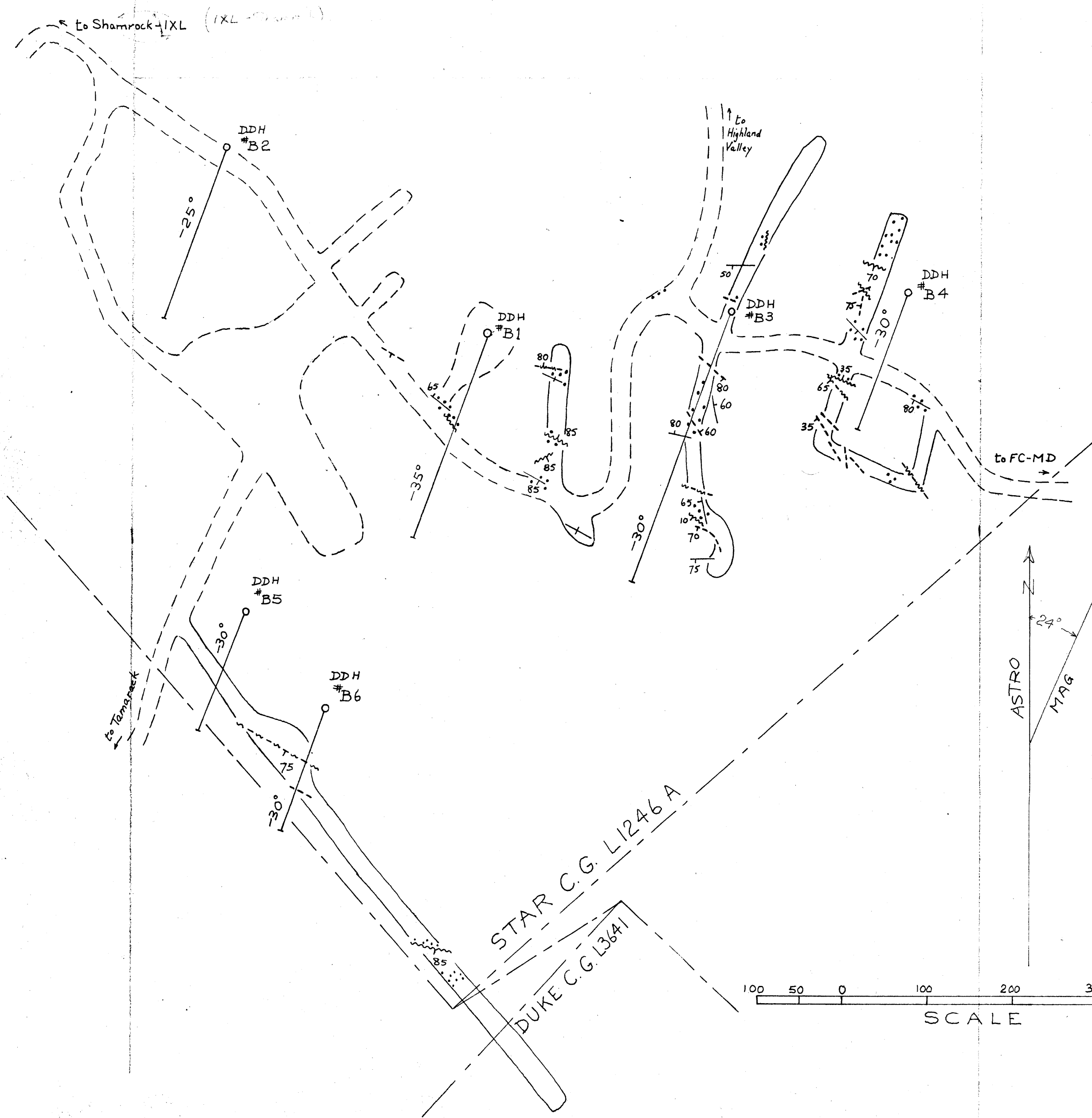
FIG- GEOLOGICAL MAP OF STAR TRENCHES, BETHSAIDA PROPERTY (partly after company maps)
