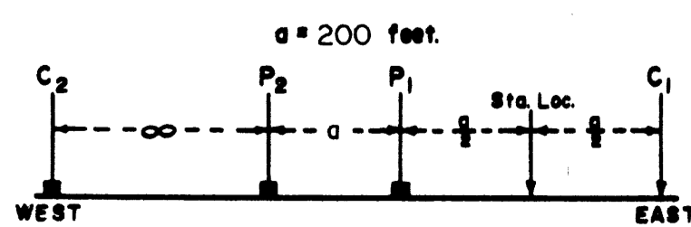
3 ELECTRODE ARRAY
