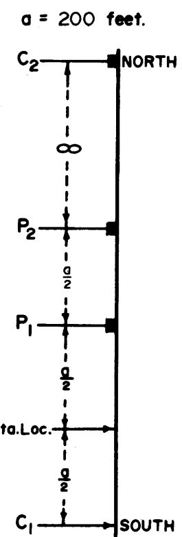
3 ELECTRODE ARRAY
