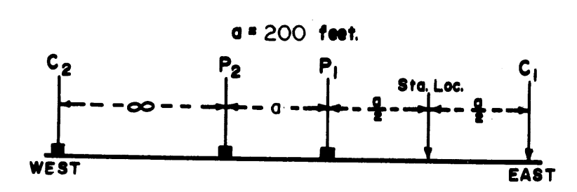
3 ELECTRODE ARRAY
