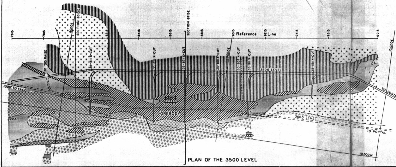
Figure 5 SIMPLIFIED GEOLOGY OF THE CRAIGMONT MINE
