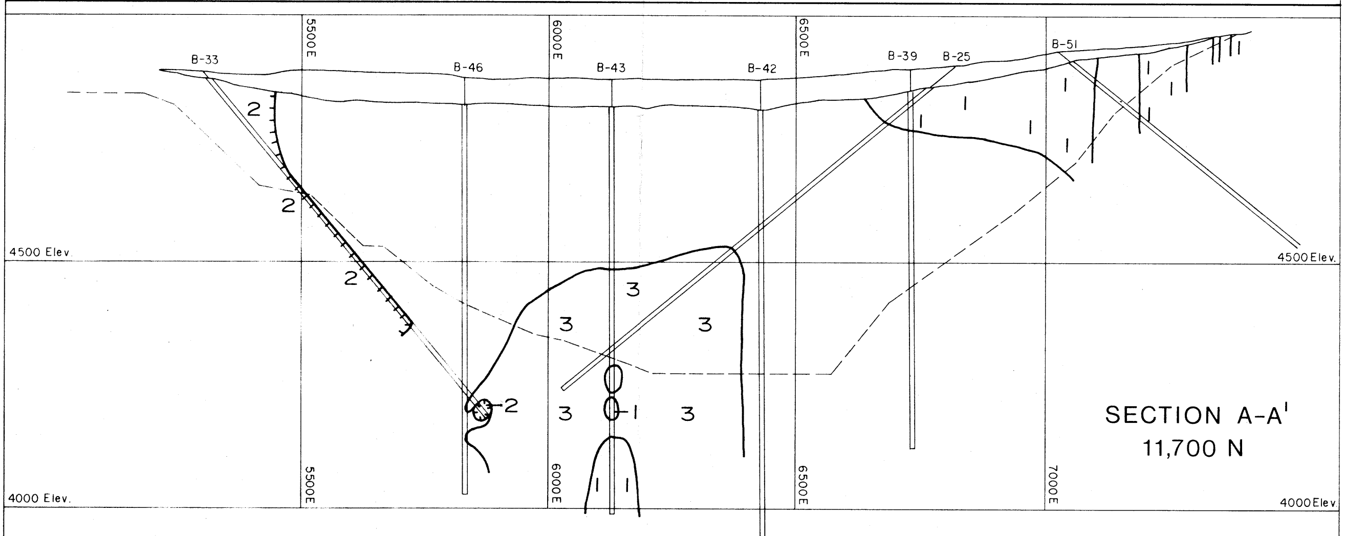
EPIDOTE & SECONDARY BIOTITE DISTRIBUTION IN THE JERSEY OREBODY
