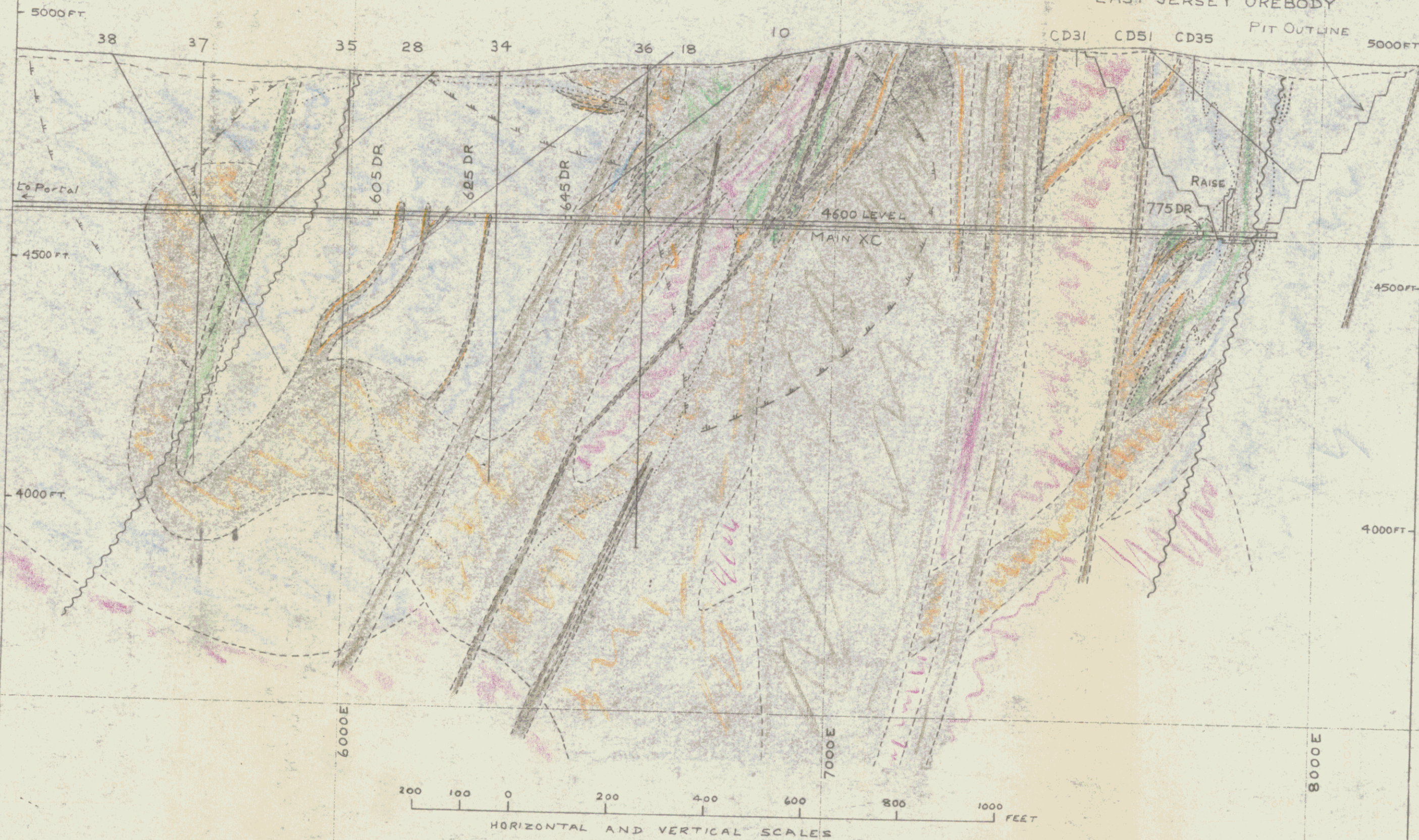
VERTICAL GEOLOGICAL SECTION ON 11400N OF THE JERSEY AND EAST JERSEY OREBODIES, BETHLEHEM PROPERTY (not all drillholes are shown) (according to information available in 1960) (for legend, see map of 4600 level)
