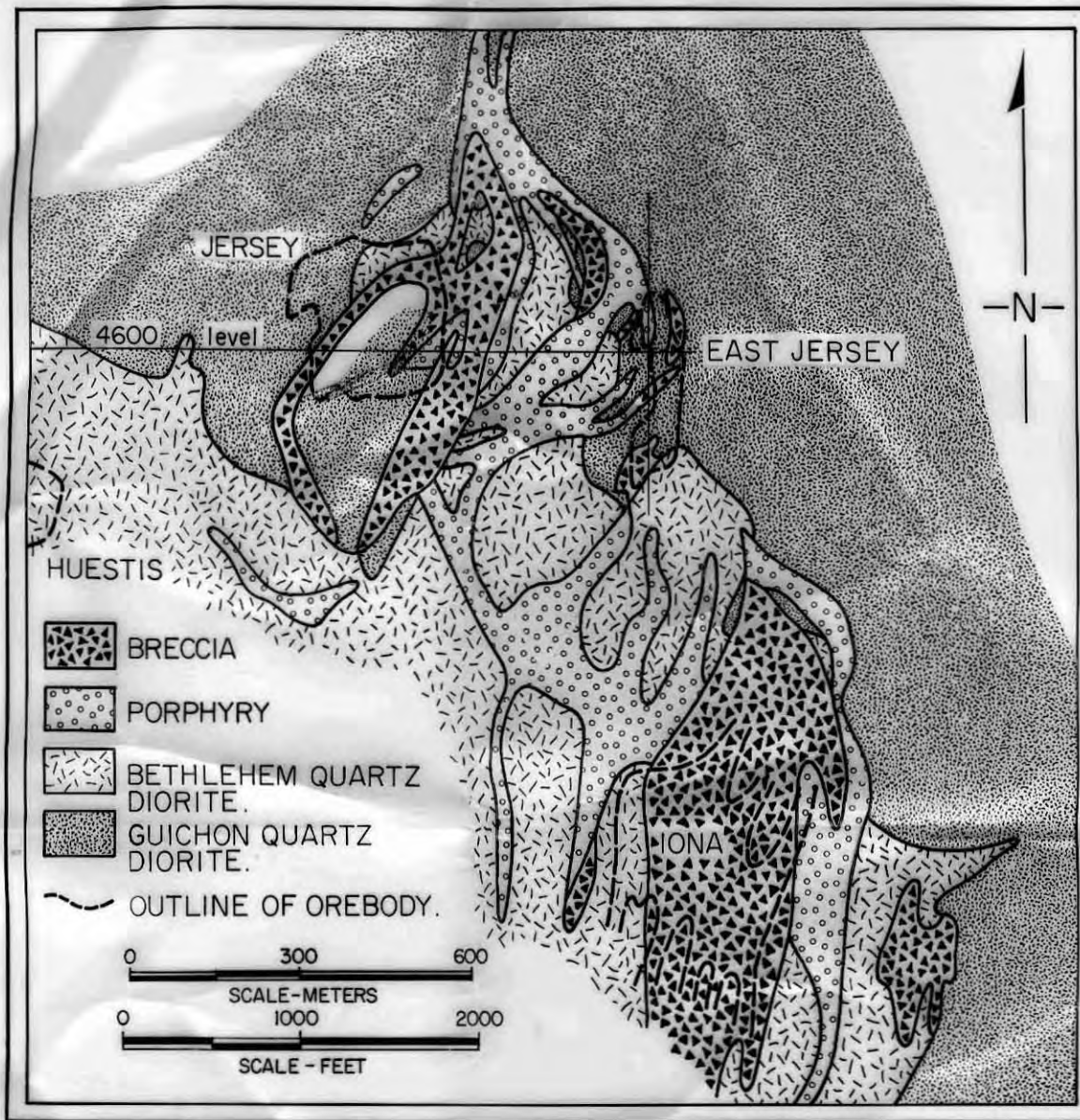
Fig. 19. Geology of Bethlehem.
