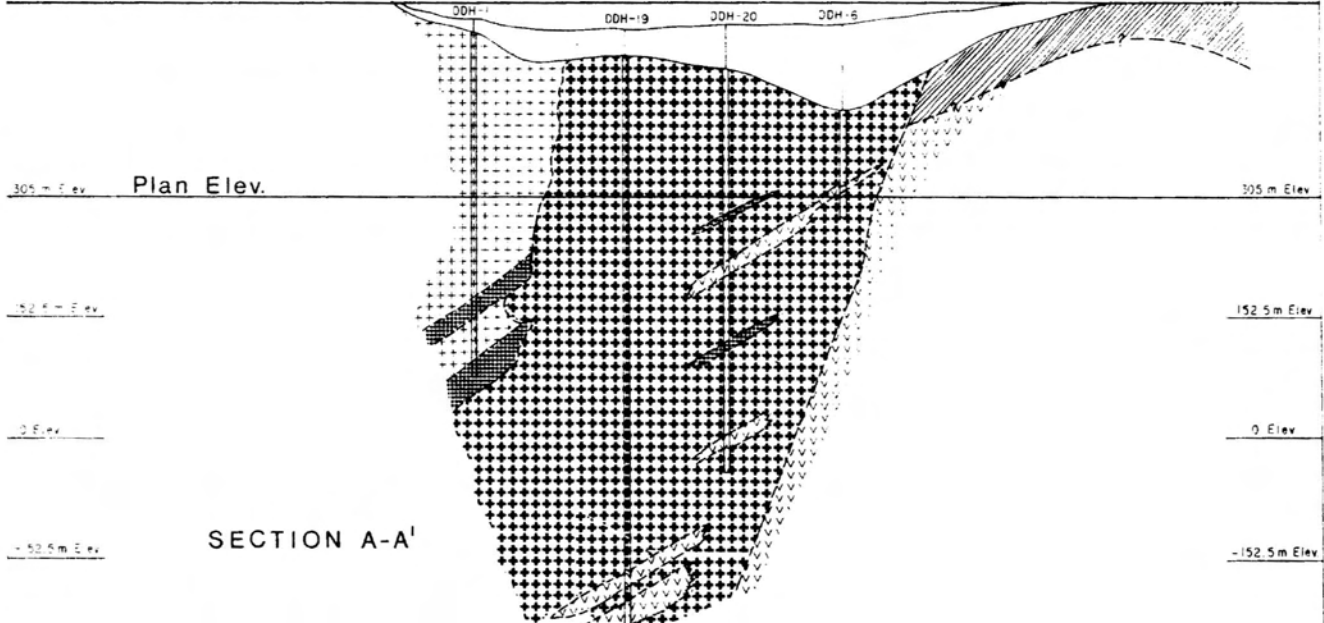
SUBSURFACE GEOLOGY OF THE MAGGIE DEPOSIT
