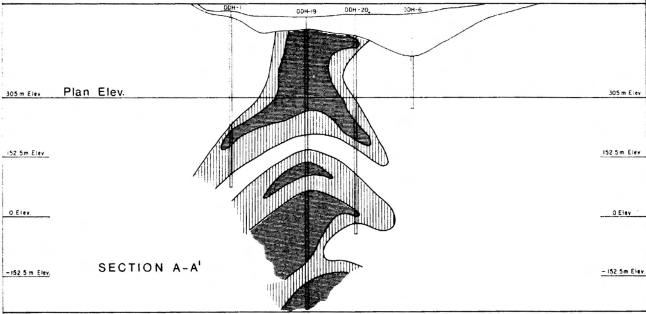
Cu-Mo DISTRIBUTION OF THE MAGGIE DEPOSIT
