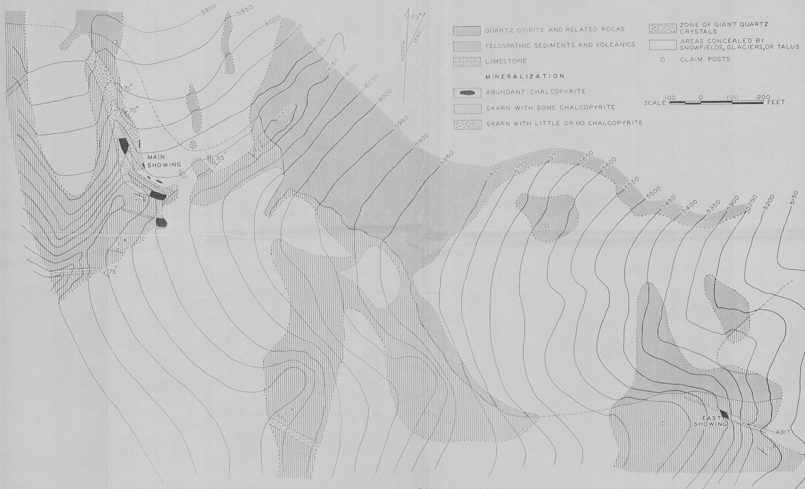
MAPPED BY W.H. WHITE, AUGUST 1949 FOR B.C. DEPARTMENT OF MINES PART OF LUCKY FOUR GROUP, CHEAM RANGE
