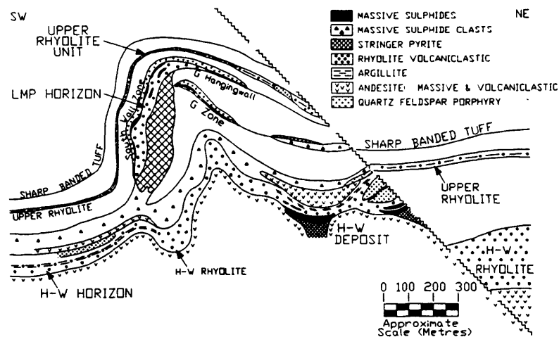
FIG 7 - Mine sequence composite cross section.
