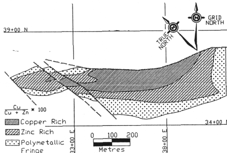
FIG 5 - H-W main lens metal zoning plan.
