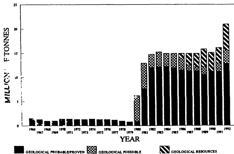
FIG 6 - Mineral inventory history Myra Falls operations.
