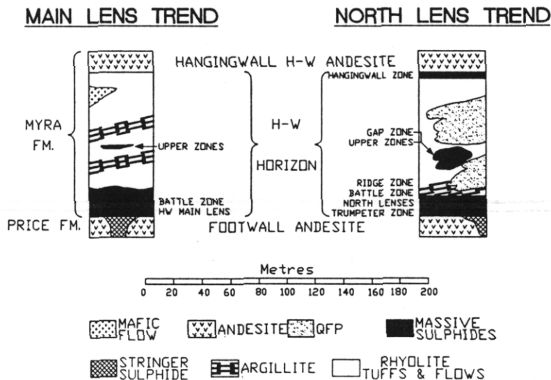
FIG 4 - Stratigraphic column H-W Horizon.
