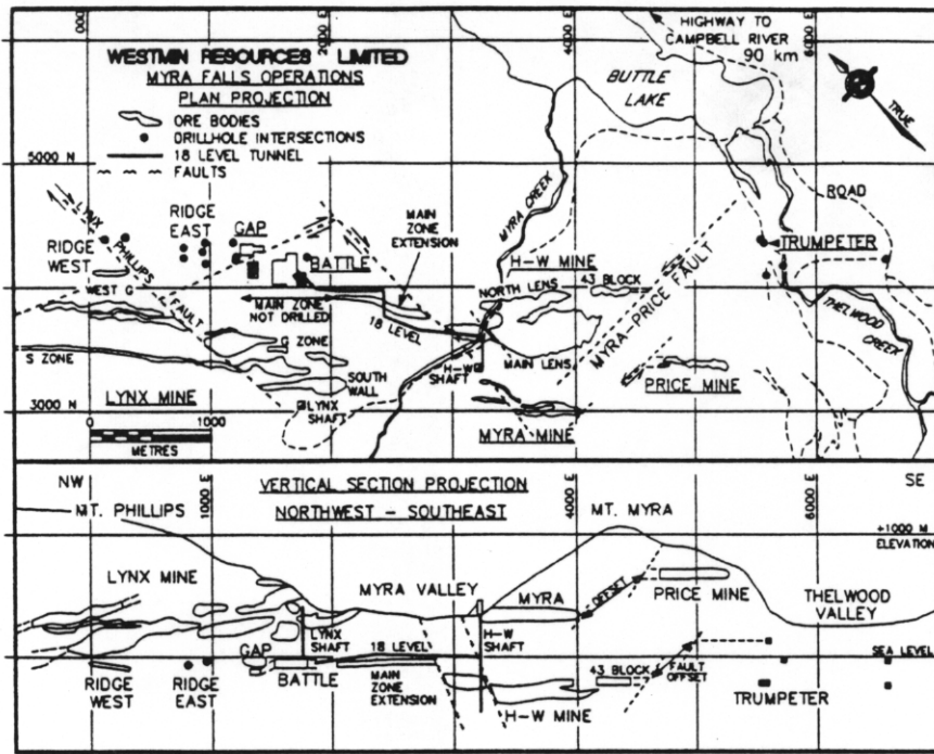
FIG 2 - Plan projection and vertical section projection.
