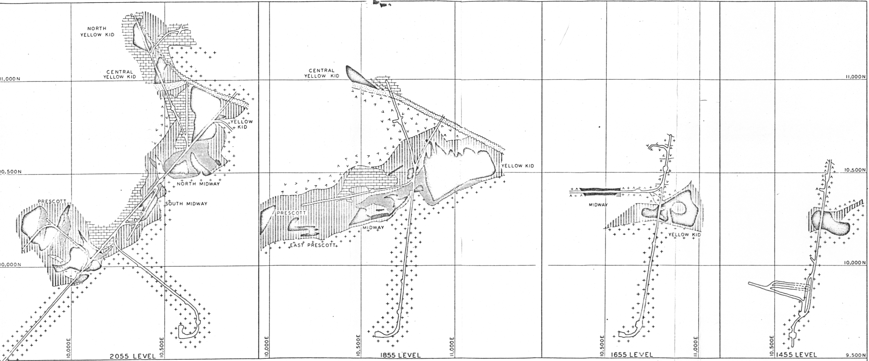
Figure 16 SIMPLIFIED GEOLOGY OF MAIN LEVELS TEXADA MINES LTD.
