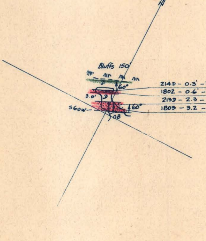
Open Cut 1520E Elev. 1055'
