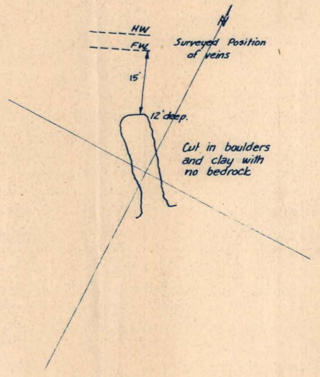
Open Cut 460E Elev. 1389'
