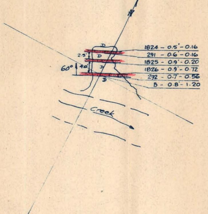
Open Cut 250E (Edmar) Elev. 1427'
