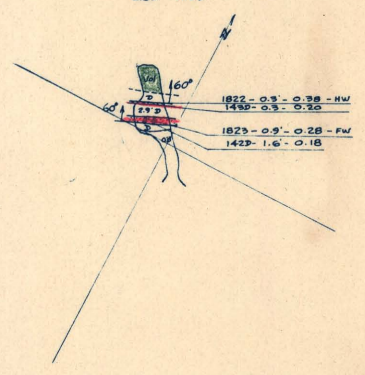
Open Cut 640E Elev. 1374'
