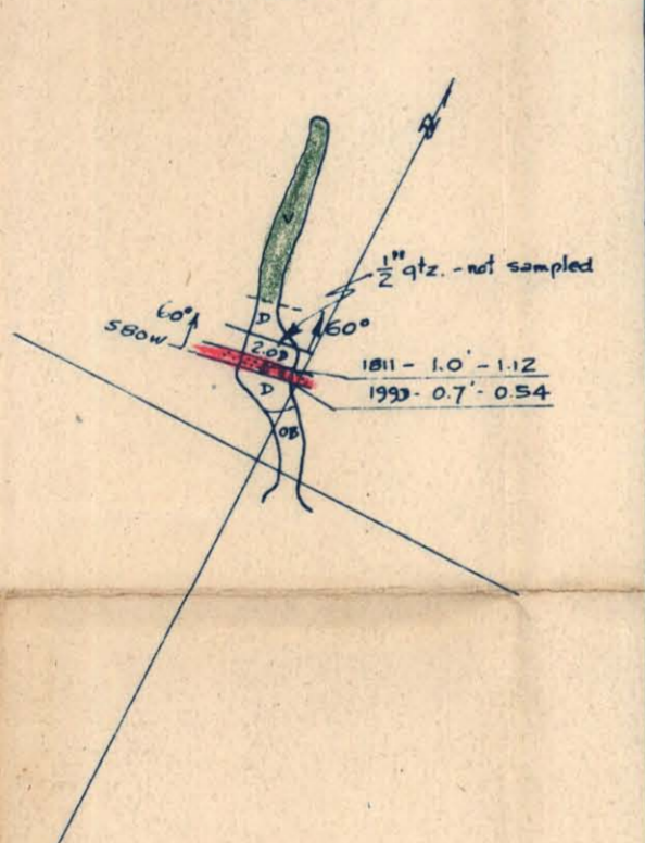
Open Cut 940E Elev. 1265'
