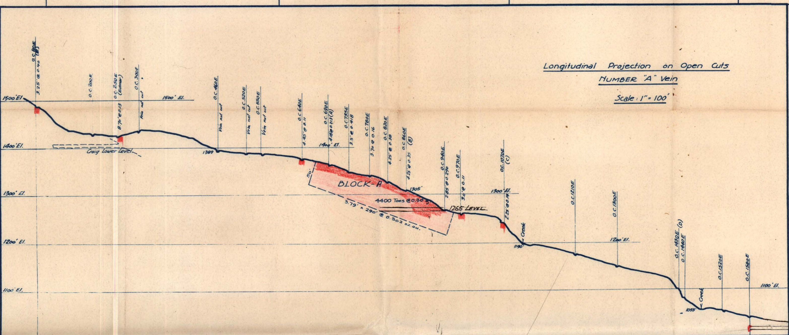
Open Cut 780E Elev. 1340'
