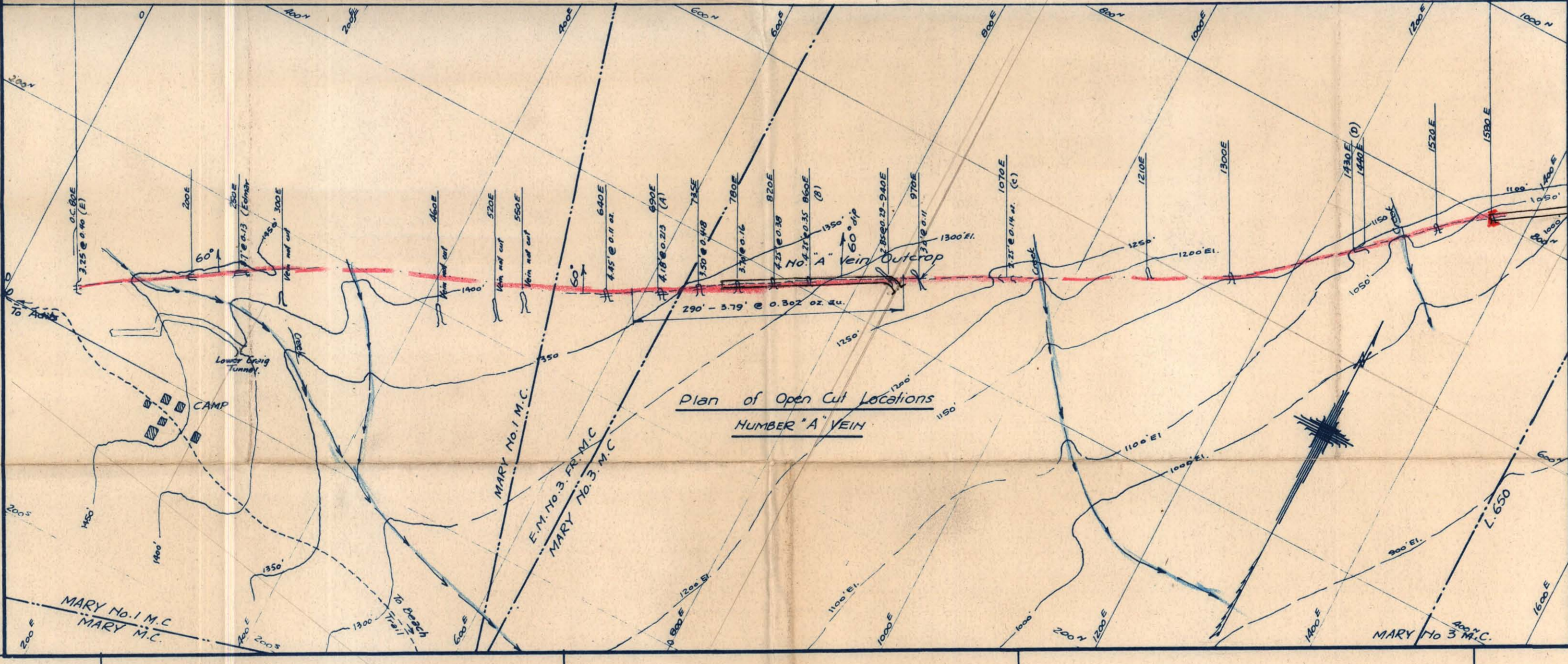
Open Cut 1300E Elev. 1148'
