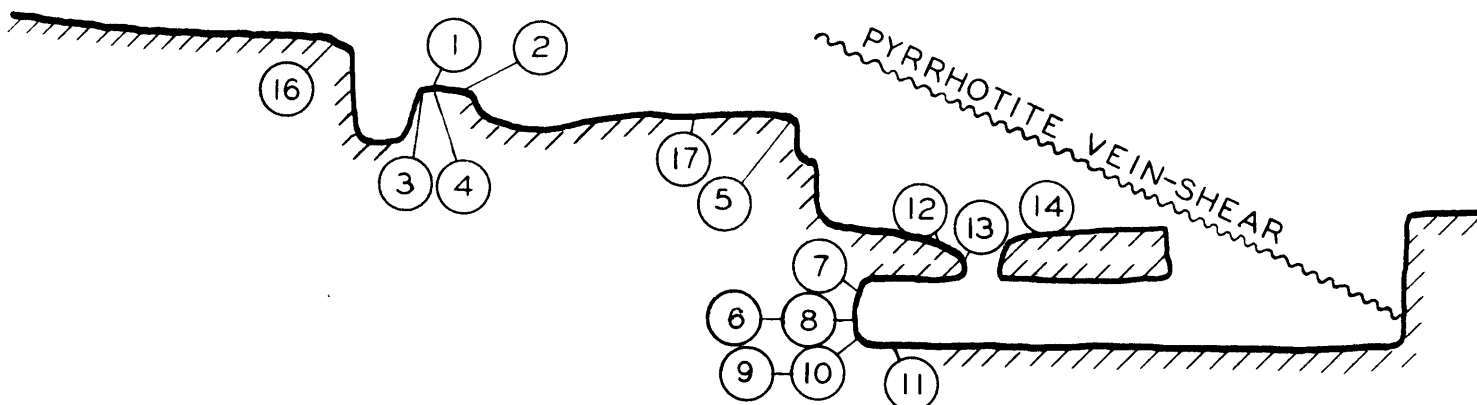
LONGITUDINAL SECTION ALONG VEIN-SHEAR
