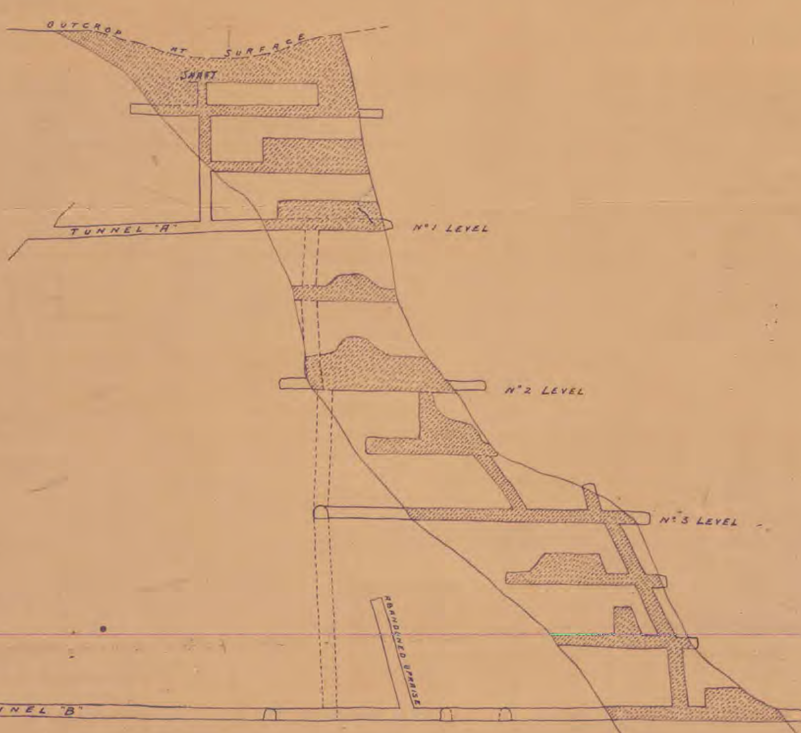
SECTIONAL ELEVATION ON LINE A.B.
