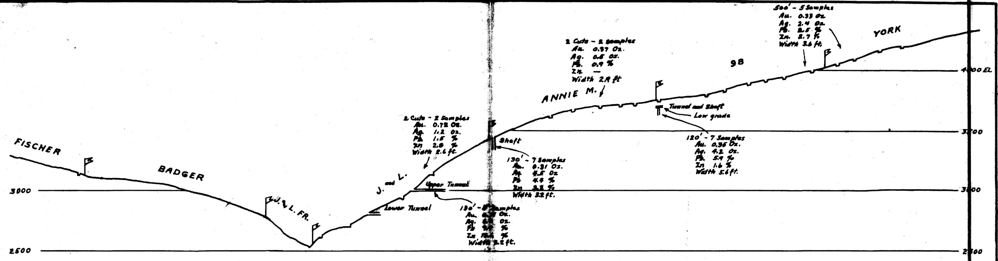
LONGITUDINAL PROJECTION ALONG VEIN. SCALE: 1" = 500'
