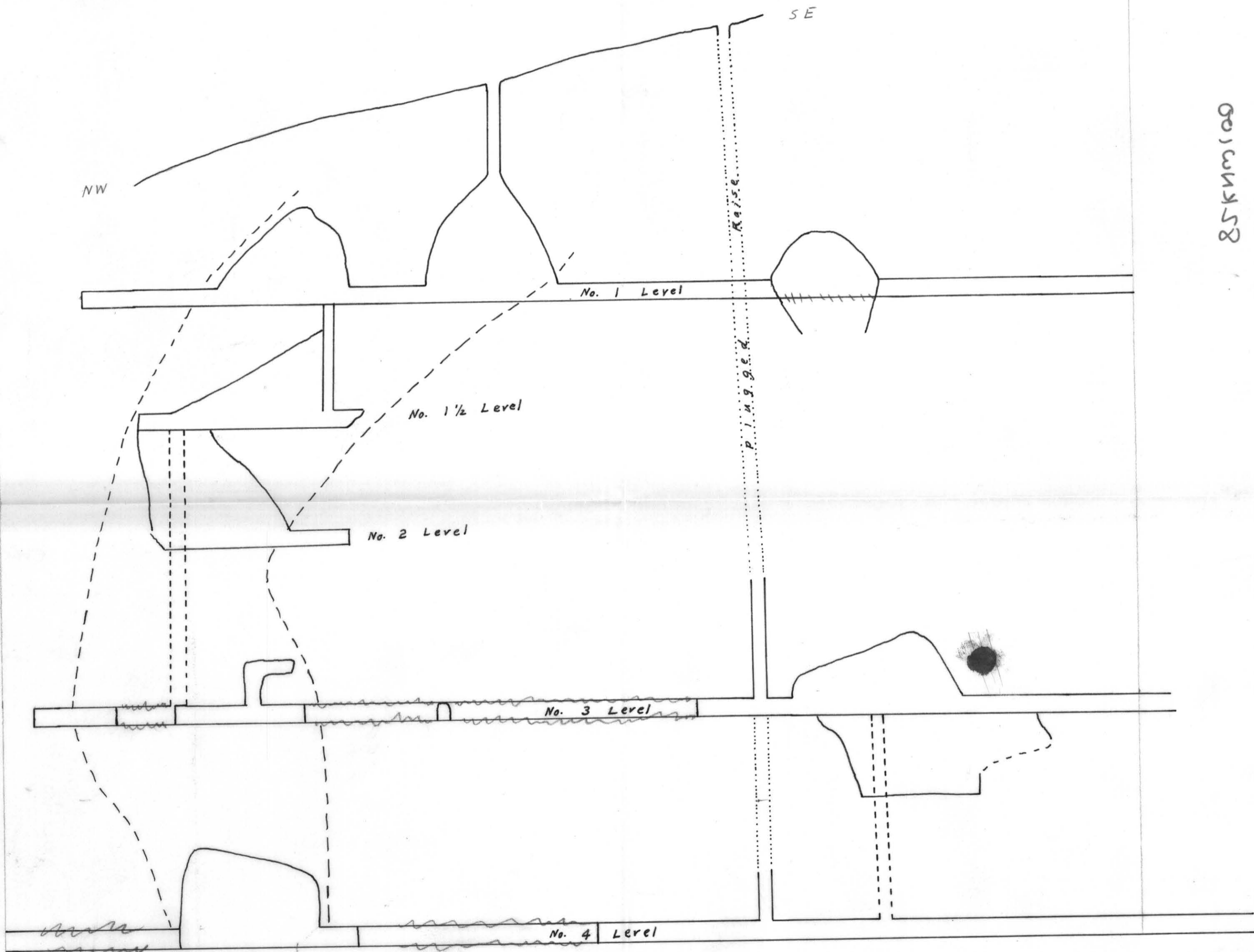
Fig. u LONGITUDINAL SECTION OF NETTIE L MAIN VEIN SHOWING STOPS & POSSIBLE OUTLINE OF NORTH MINERALIZED BODY 1" = 30'
