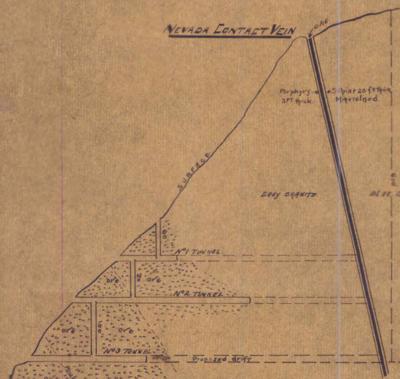
SECTIONAL ELEVATION SHOWING TUNNELS N°1, N°2, N°3, ON THE ROYAL CANADIAN VEIN WITH THE NEVADA CONTACT VEIN Scale 100 feet to the inch
