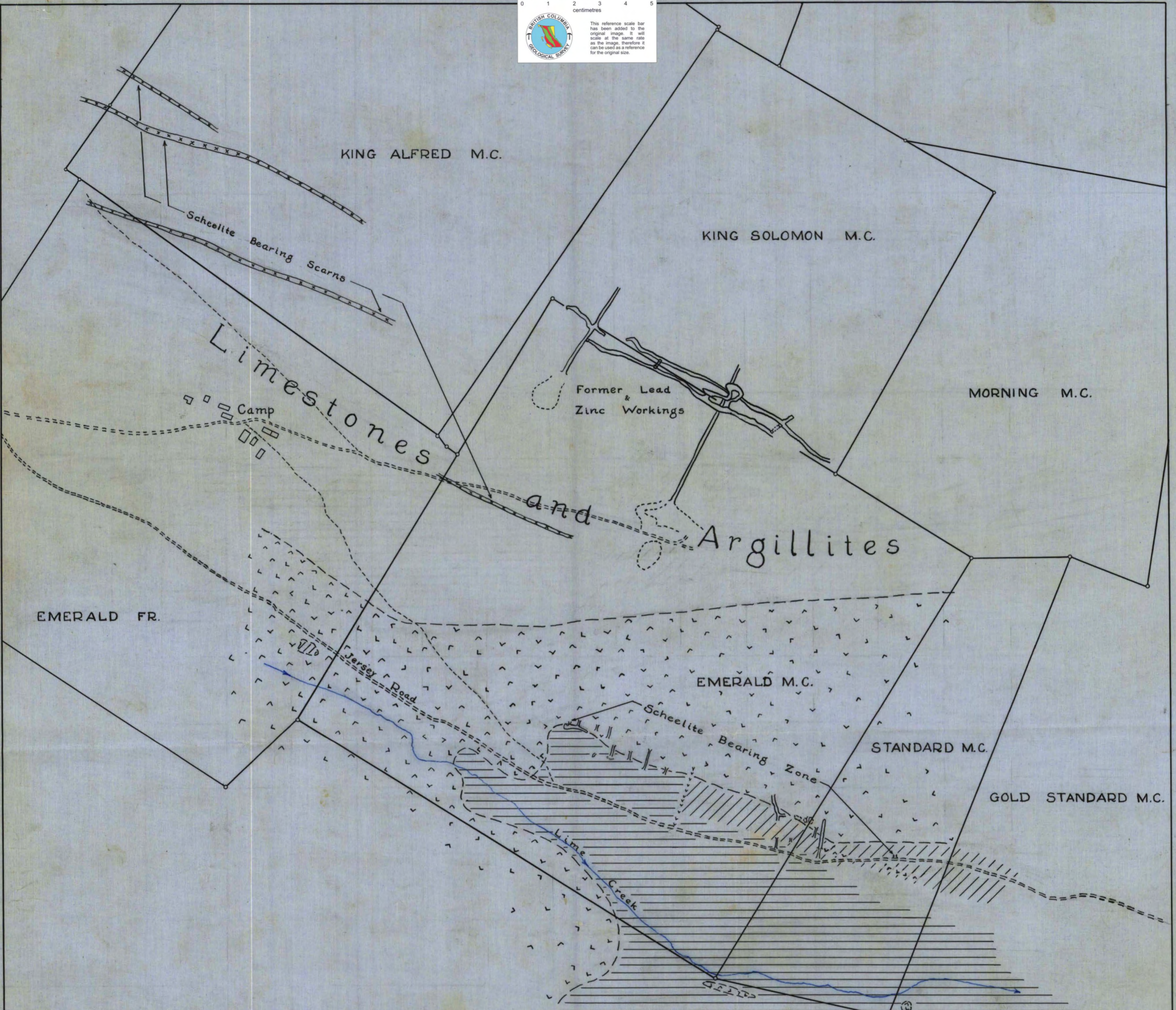
SKETCH MAP OF EMERALD PROPERTY SHOWING ESSENTIAL GEOLOGY OF SCHEELITE BEARING ZONE
