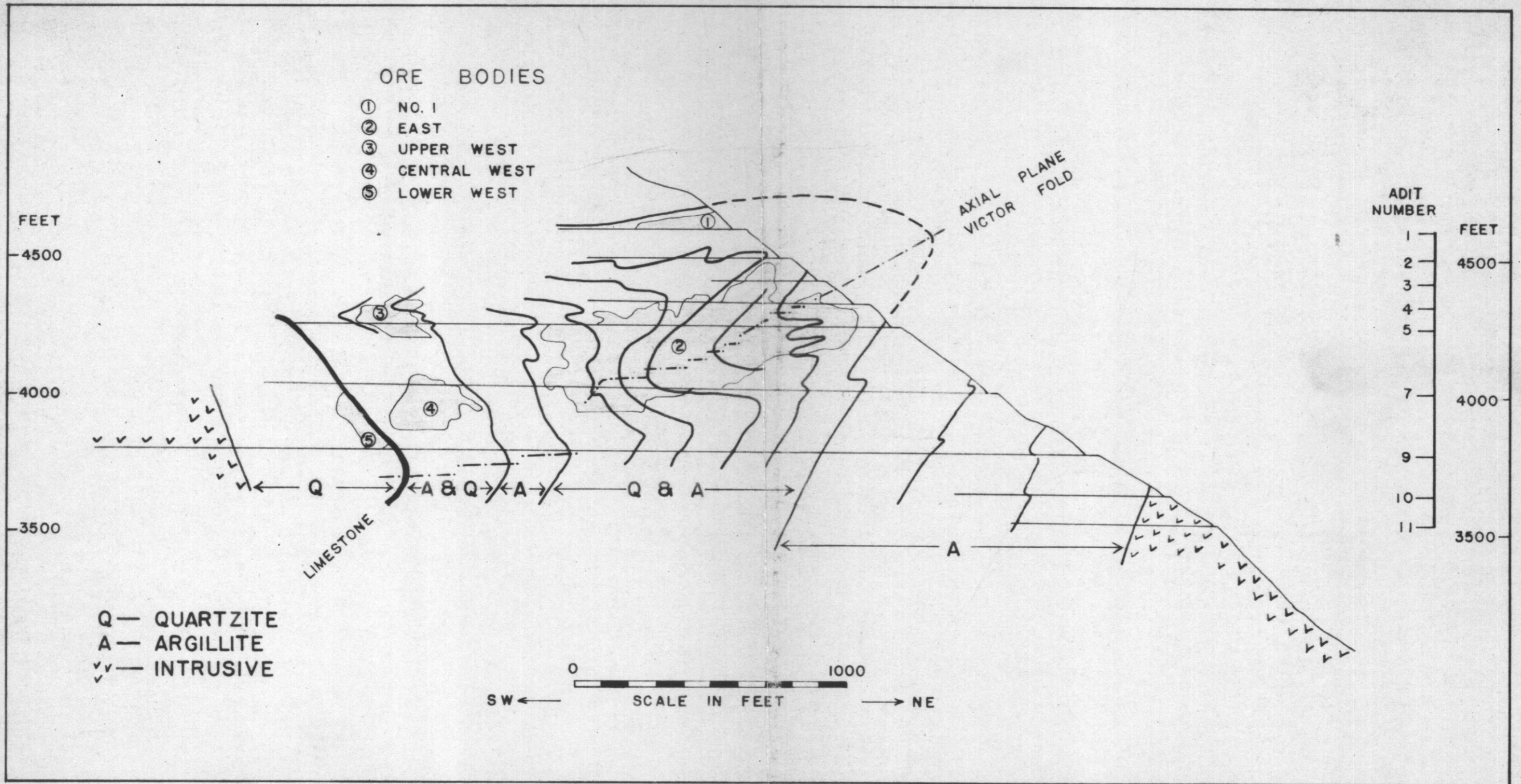
FIGURE 1. A LONGITUDINAL SECTION SHOWING THE VICTOR FOLD AND THE DISTRIBUTION OF THE ORE BODIES
