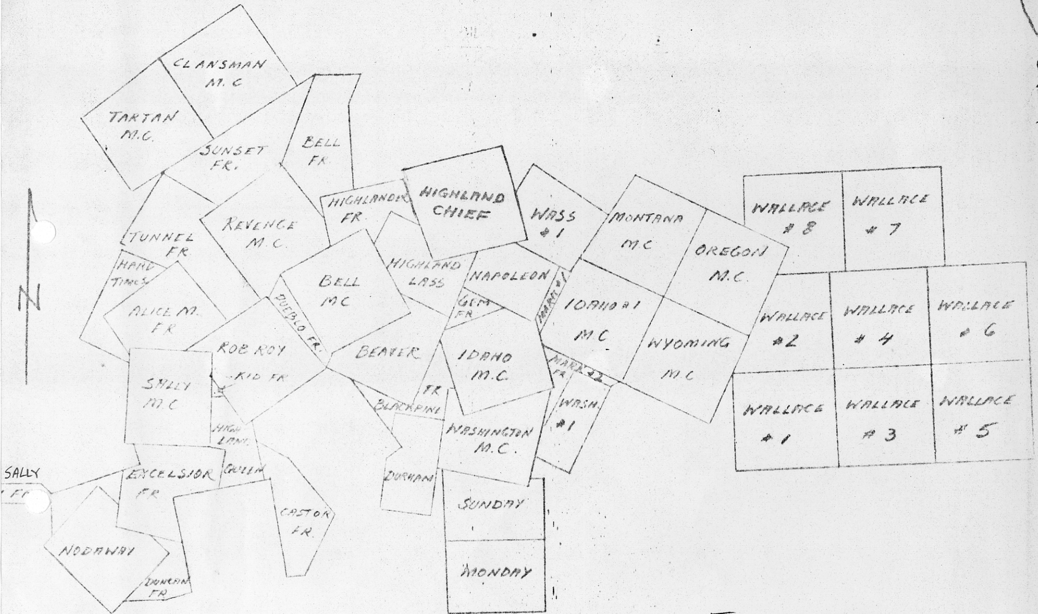
TECK CORPORATION LTD BEAVERDELL, B.C. SKETCH SHOWING CROWN GRANTS AND RECORDED CLAIMS AT BEAVERDELL, B.C.
