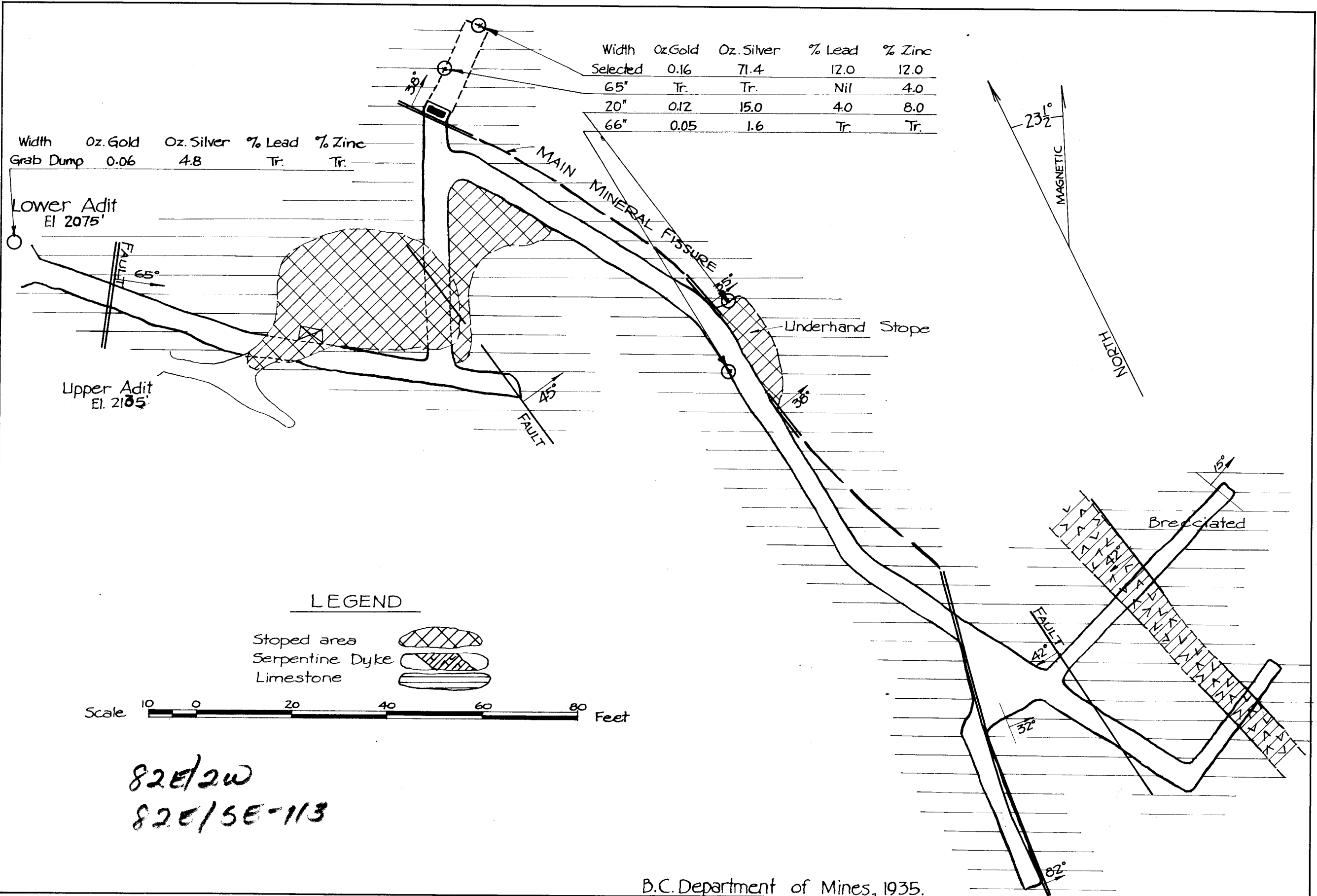
Plan Imperial Mine Underground Workings, Greenwood M.D.
